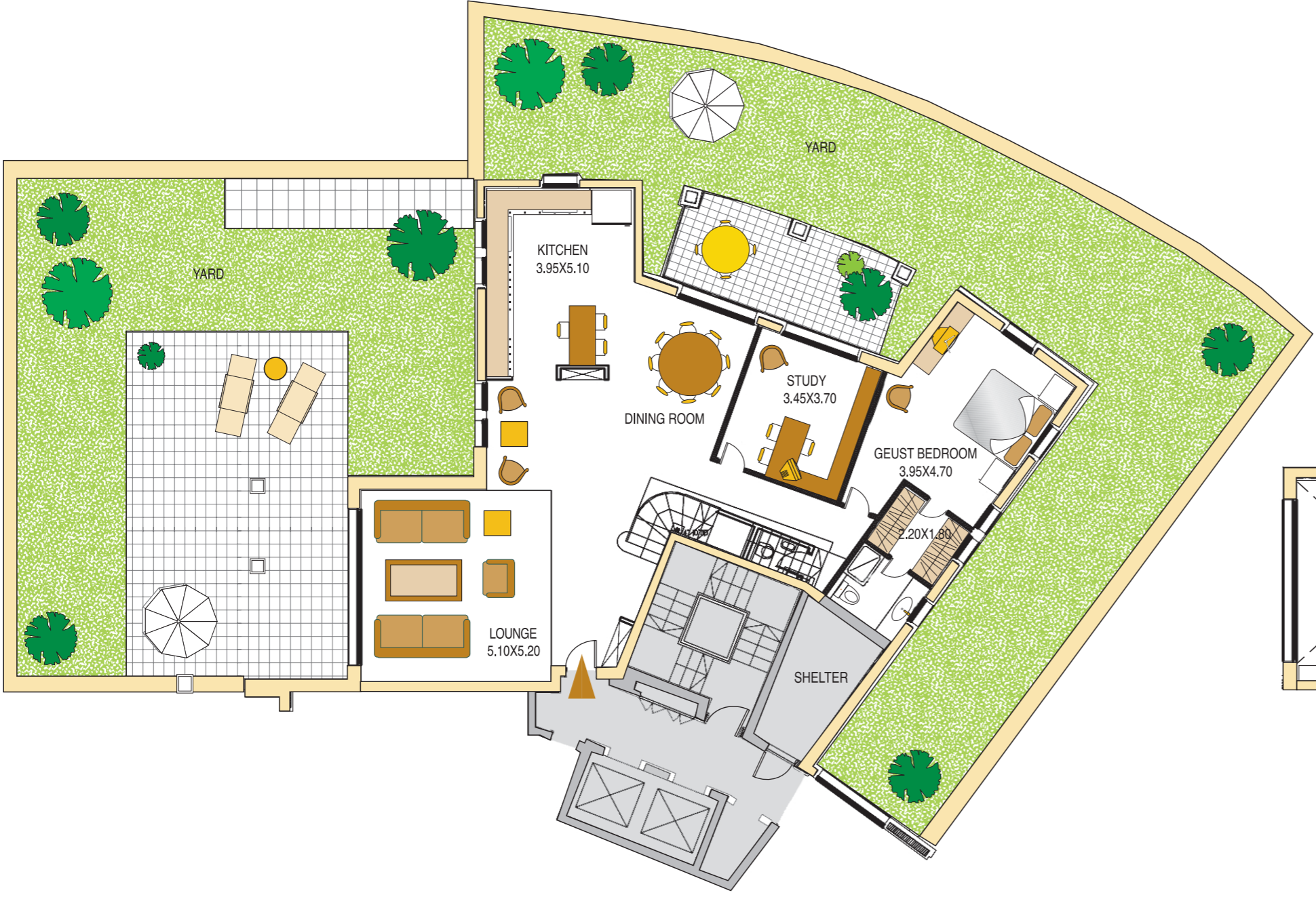
GROUND FLOOR
